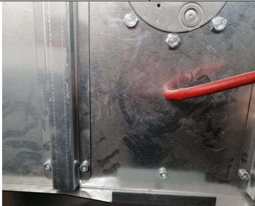
Photo 8. Cable Entry
